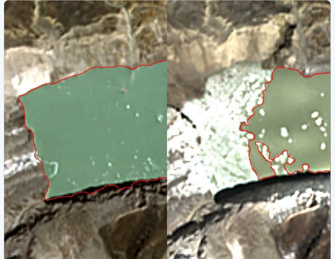
South Lhonak Lake, Sikkim — before and after the October 2023 outburst
