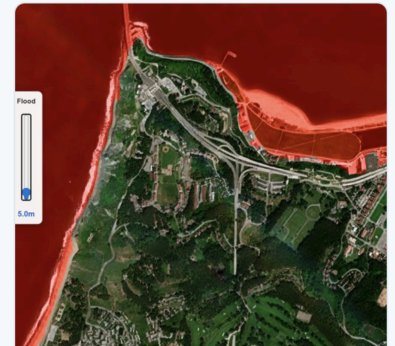
Sydney, Australia — flooding at 5m above sea level
