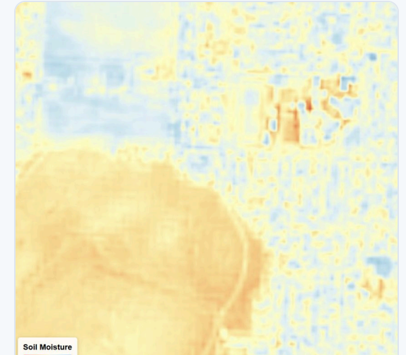
Nevada, USA — soil moisture at 2m
