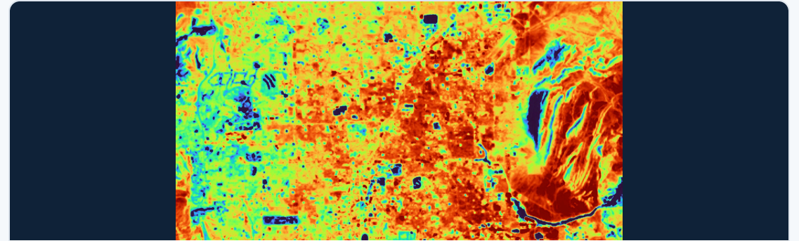
Las Vegas, July 2025 — 25m surface temperature (Landsat-8/9 band 10); parks, lakes and irrigated land cool, desert and roofs hot
