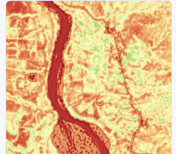
Pampas, Uruguay — grassland biomass at 2m
