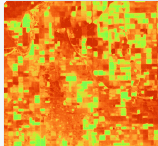
Imperial Valley, California — farm fields at 25m (Landsat-8/9 band 10), 15 Aug 2026
